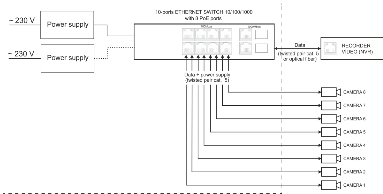
Fig. 1. Block diagram.
